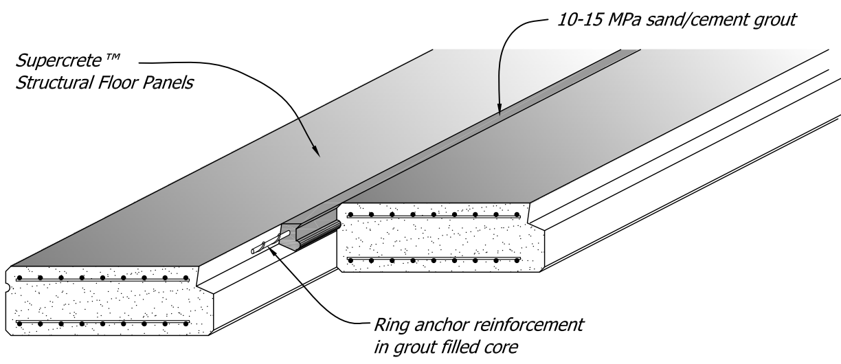
Floor Panel & Ring Anchor Isometric Detail
