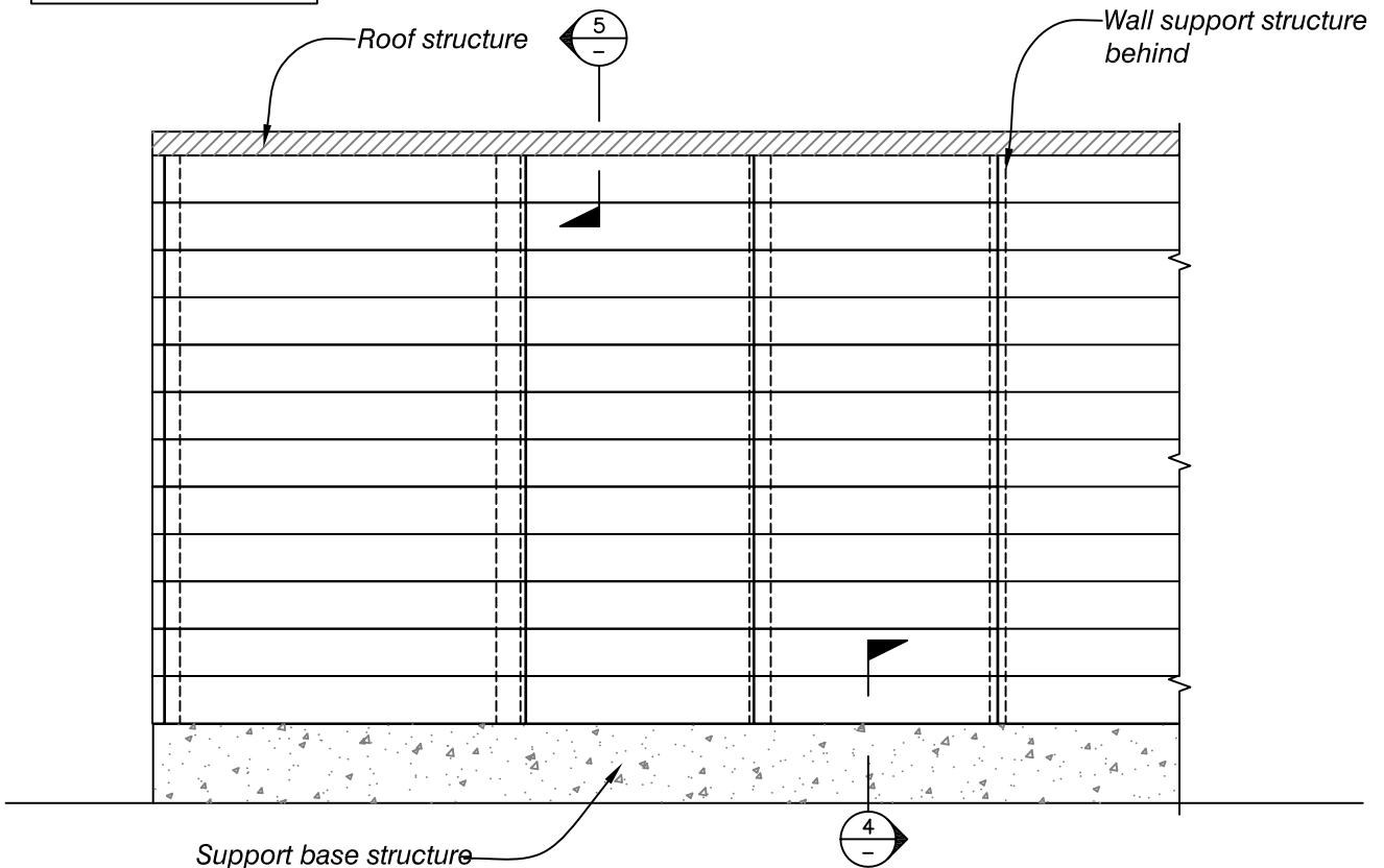
Elevation View - 1
