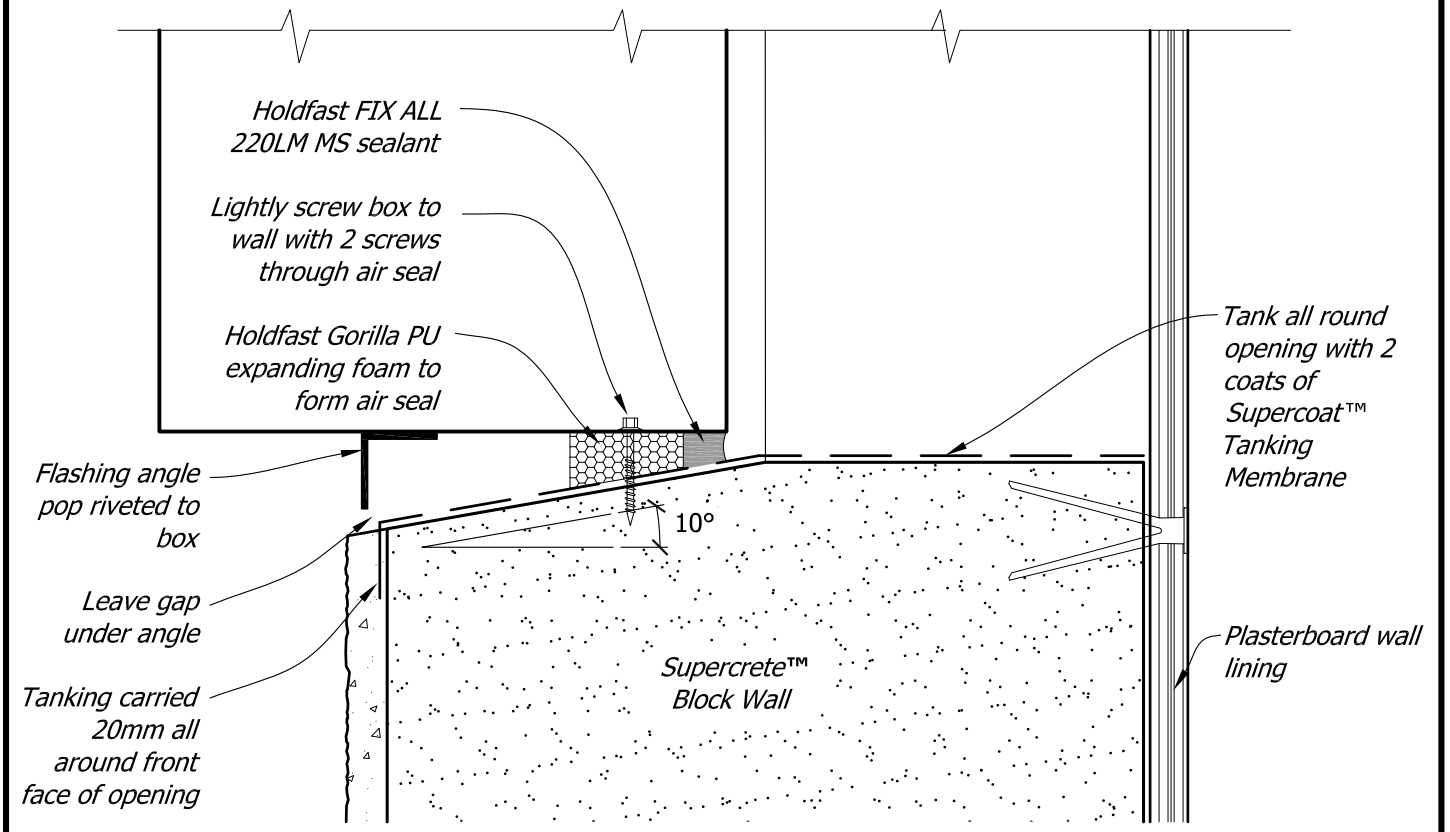
Section at Sill
