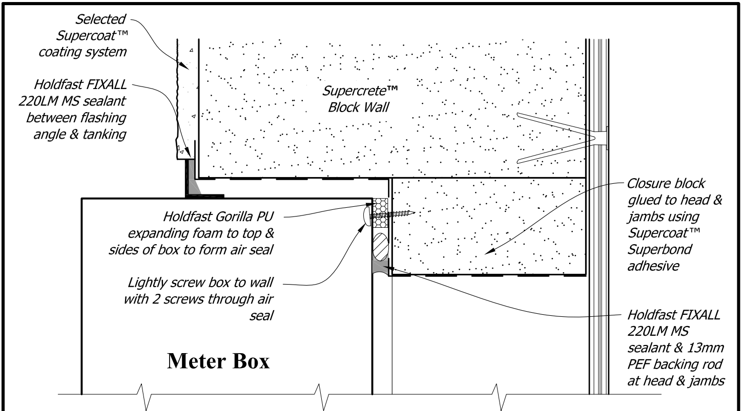
Section at Head Jamb section similar
