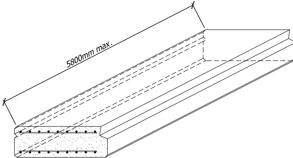
Floor Panel Isometric Detail
