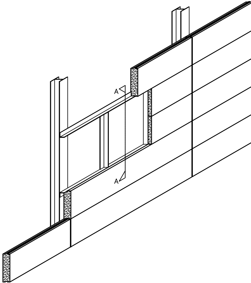
Isometric View
